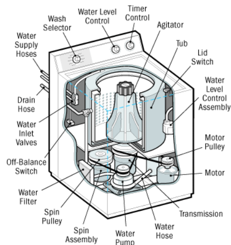
Figure 2: Diagram of a top loader washing machine.
